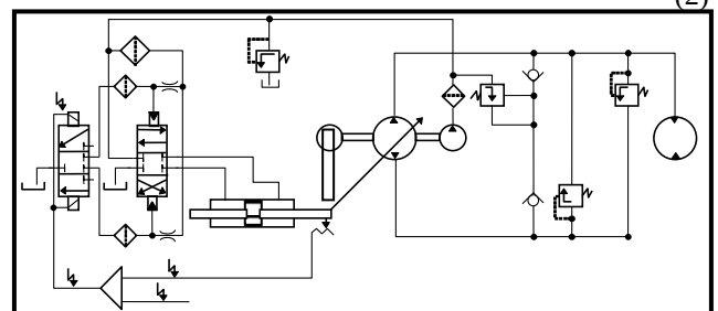
Figure 1. Electro-hydraulic system
